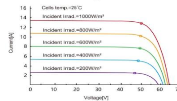
Current-Voltage Curve
